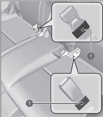
① Loop
