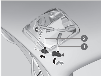
1 Socket 2 Bulb
