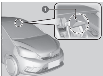
1 Front Wide View Camera
