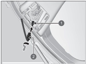
1 Bulb 2 Socket
